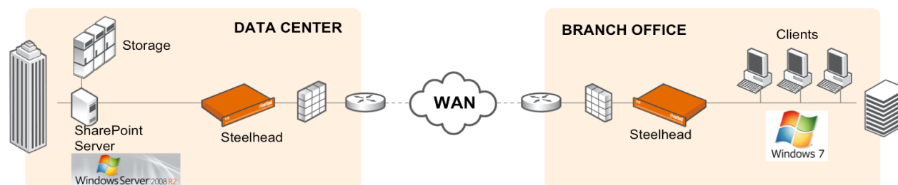
Figure 1: Deployment Diagram, WAN-T1 with 100ms Latency setup
