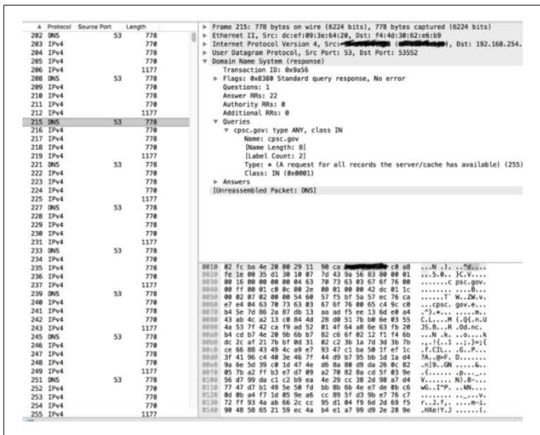
Figure 3-5. DNS amplification packet
